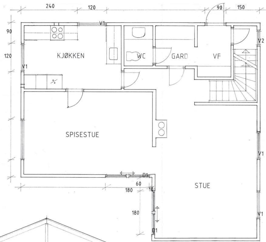
PLAN 1 ETG
